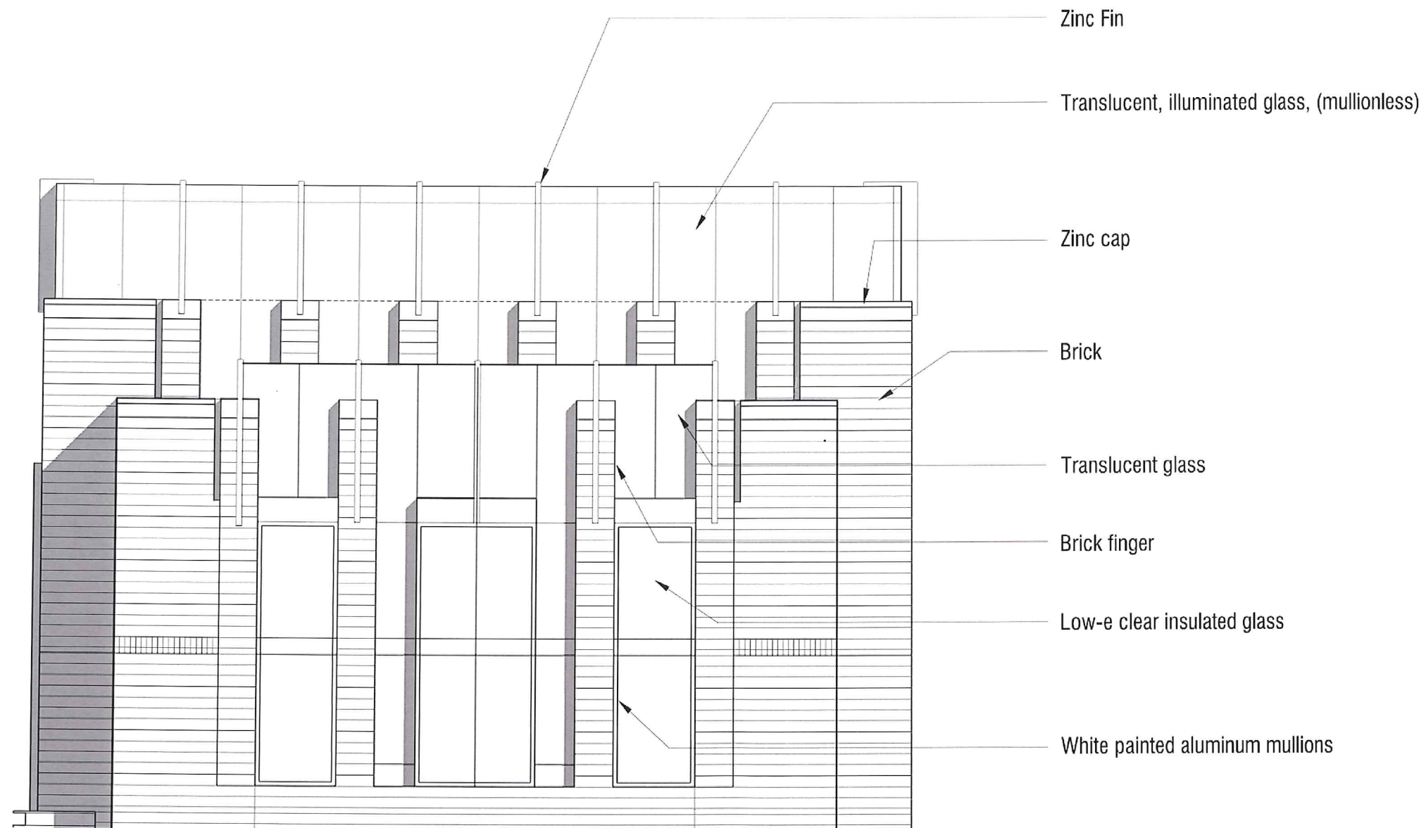
Enlarged Elevation Penthouse at Water St.
