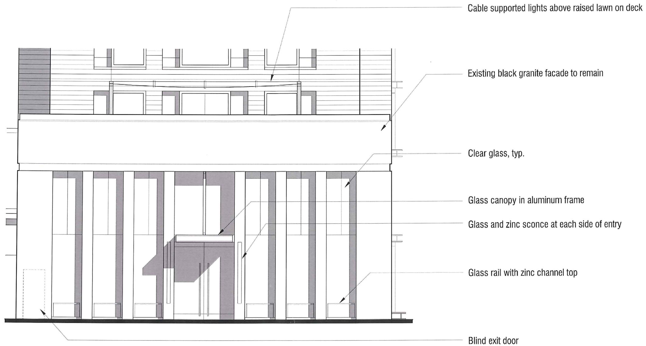
Enlarged Elevation Existing facade at Main St.
