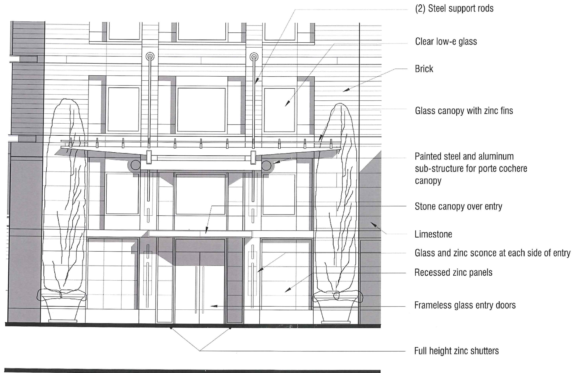
Enlarged Elevation Porte Cochere at Water St.
