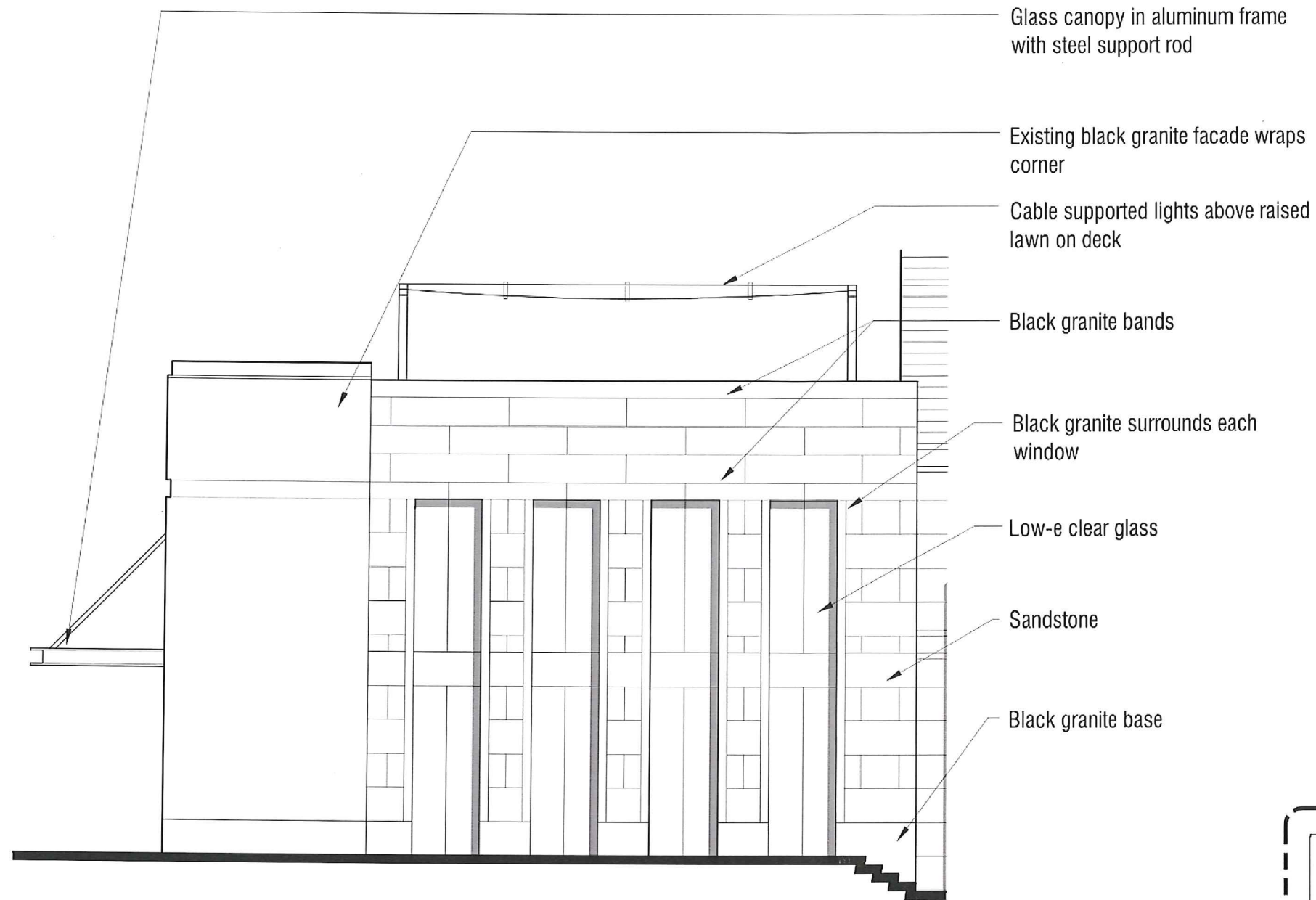
Enlarged Elevation Restaurant at Second St.
