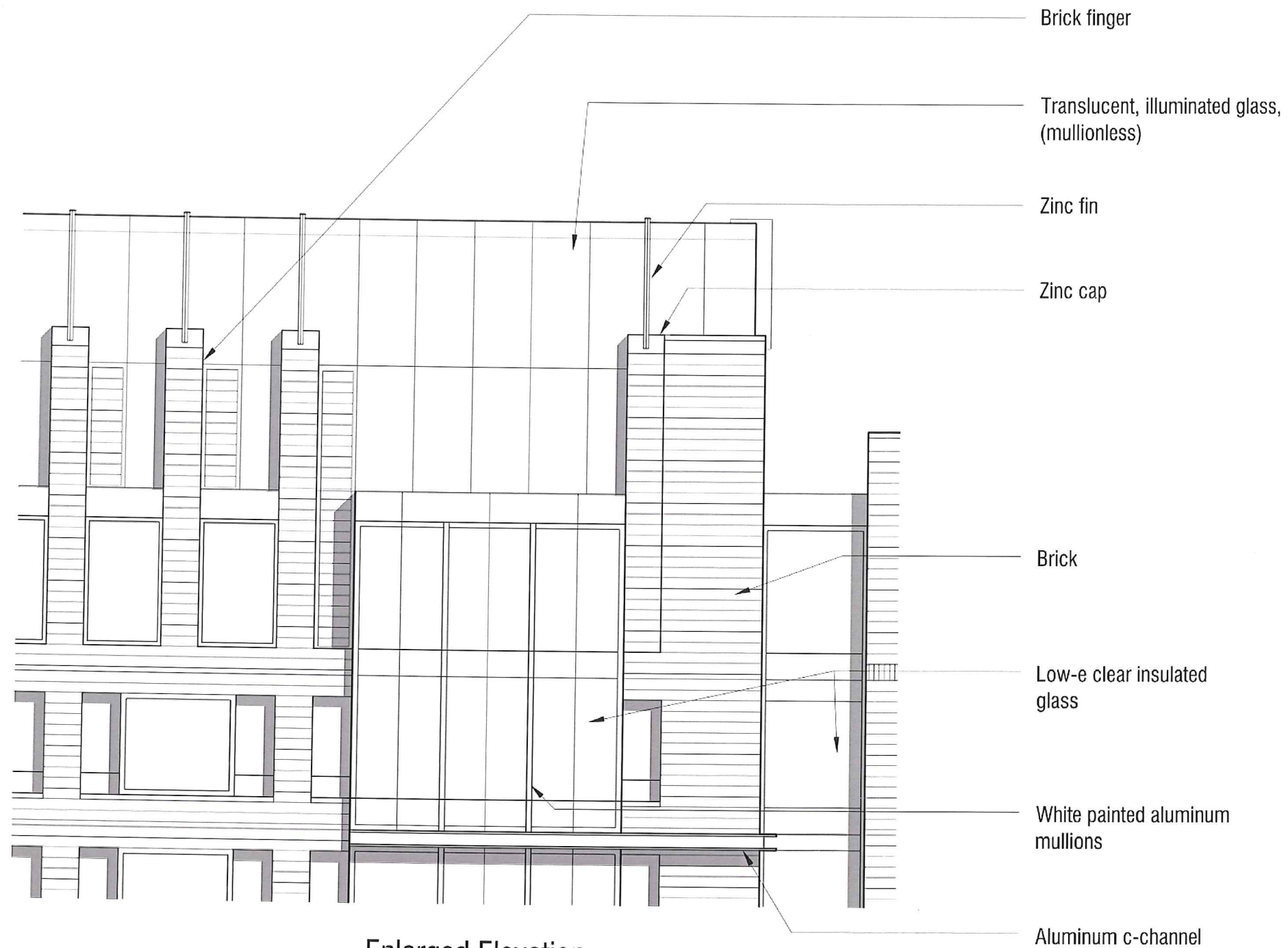
Enlarged Elevation Penthouse at 2nd St.
