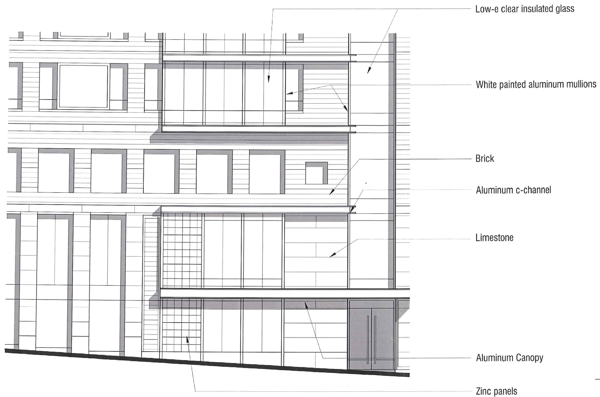
Enlarged Elevation Ground Level at 2nd St.
