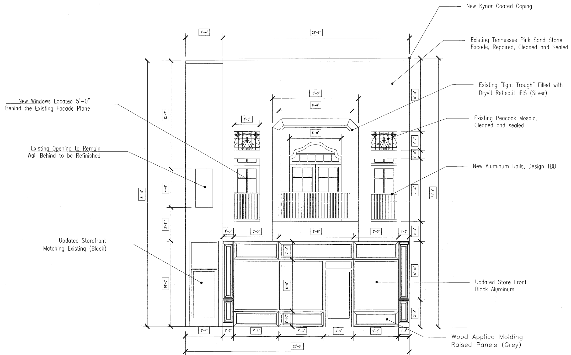
102 South Main Street Facade (Snooky's) Scale \frac{3}{8}" = 1'-0"
